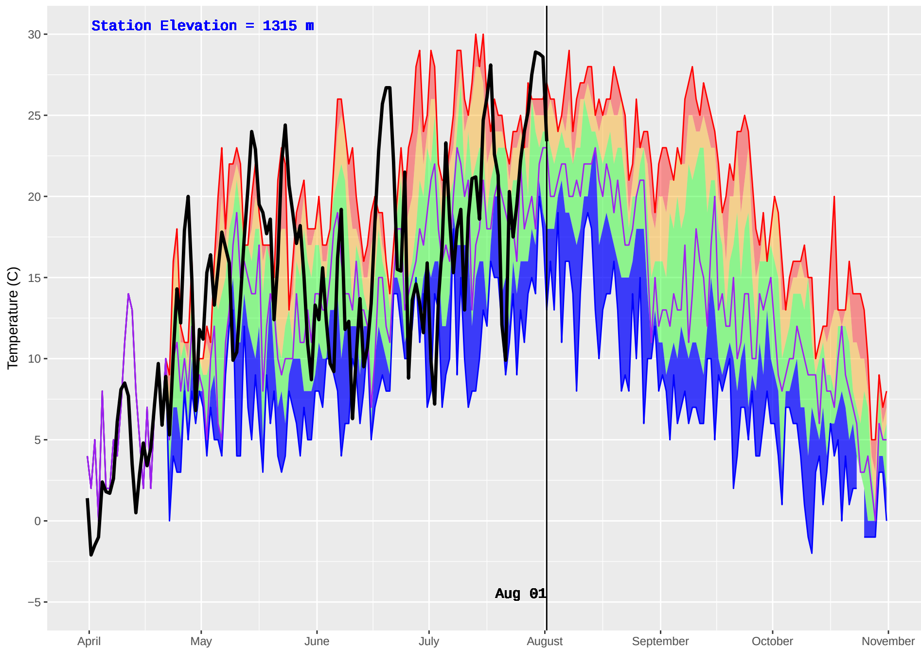
MAYSON (1082) : Historical (2010–2016) and Current (2018) Daily Temperature
