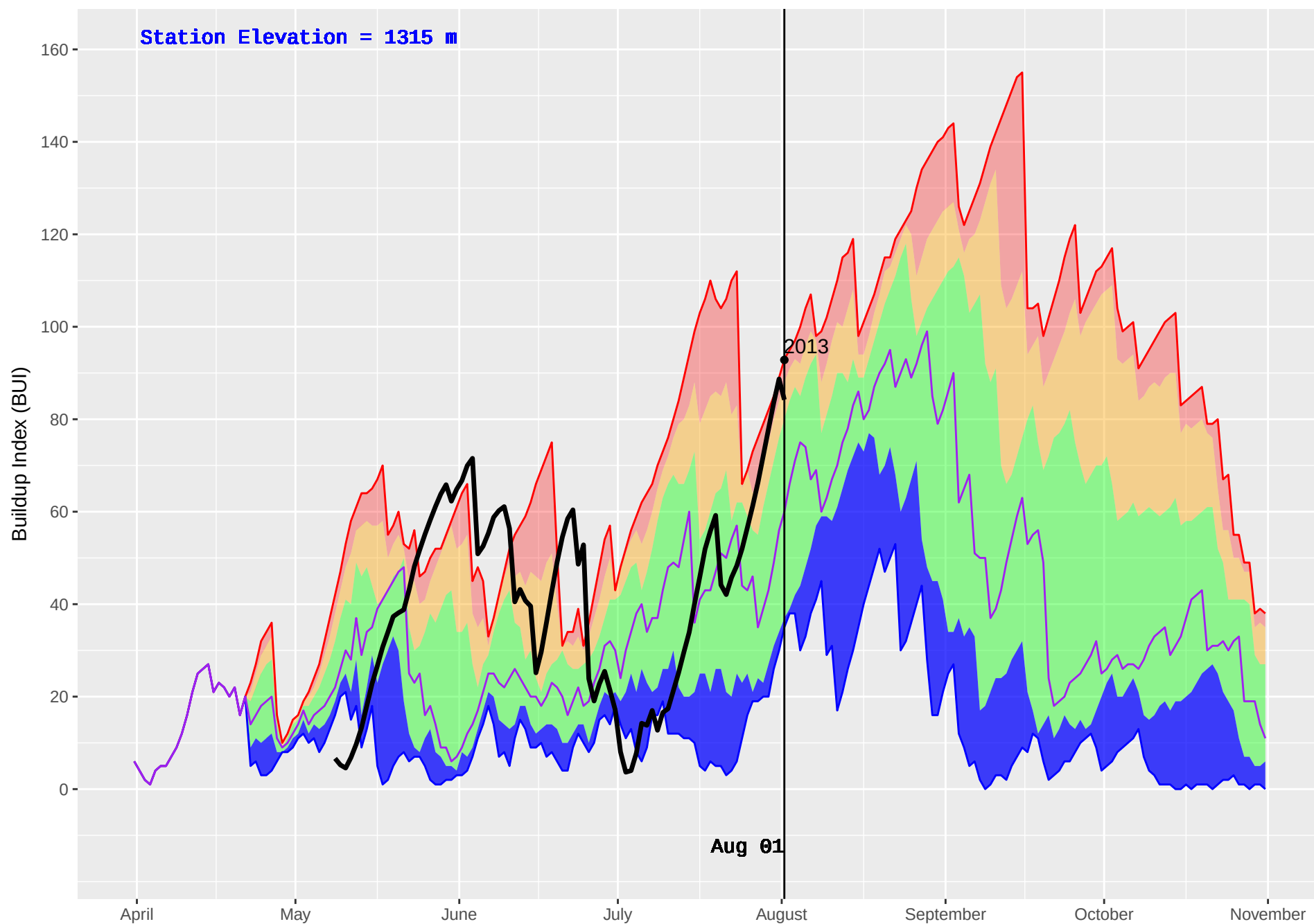
MAYSON (1082) : Historical (2010–2016) and Current (2018) Daily Buildup Index (BUI)
