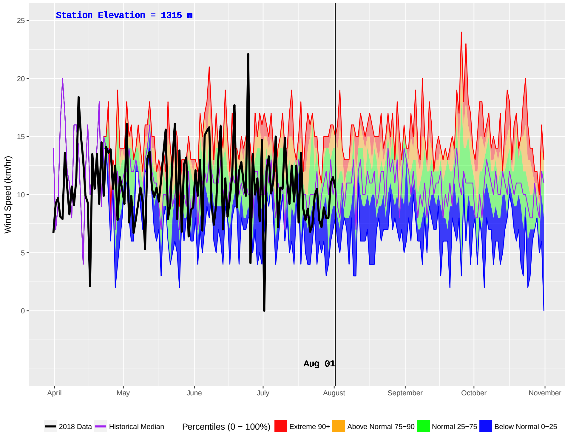
MAYSON (1082) : Historical (2010–2016) and Current (2018) Daily Wind Speed
