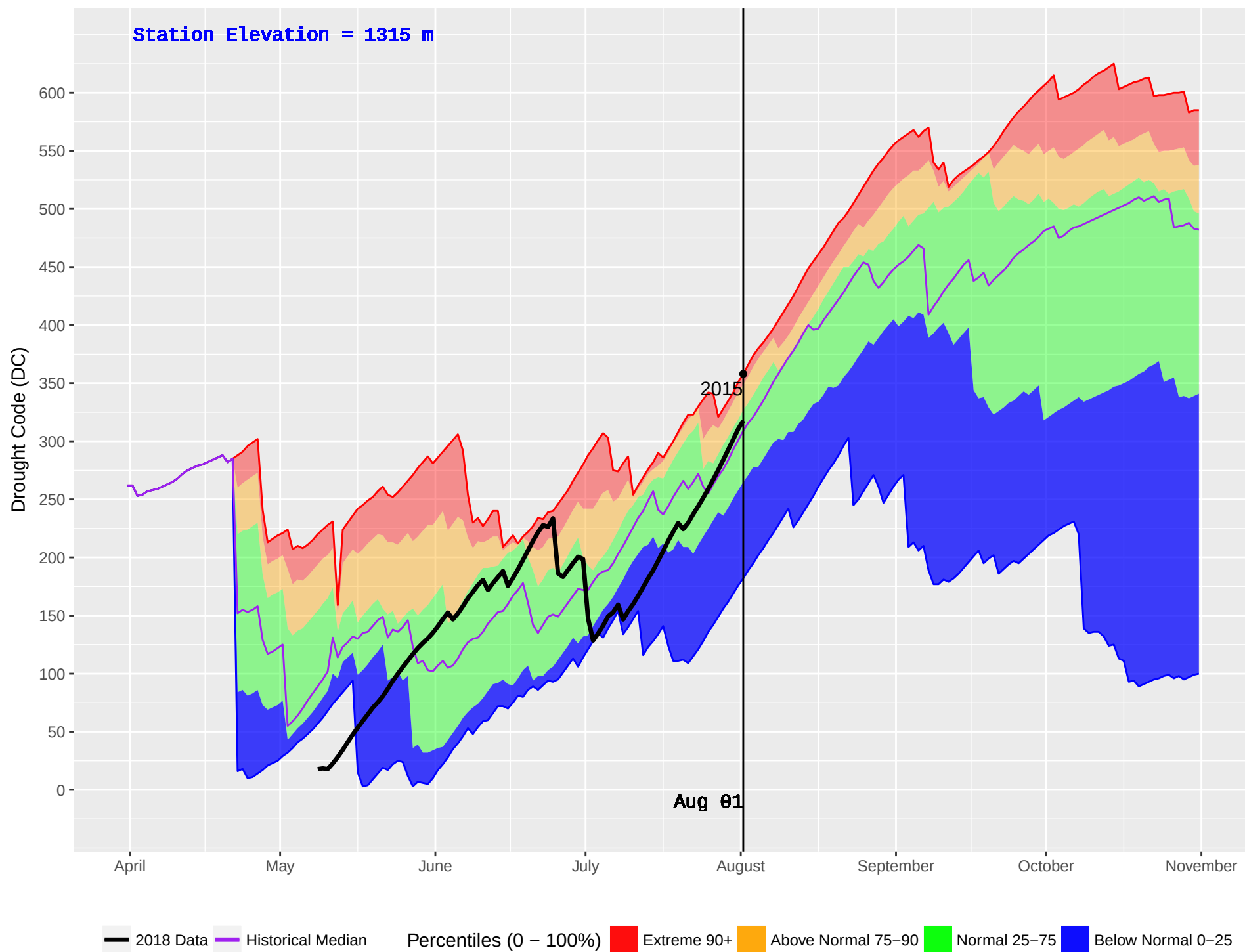
MAYSON (1082) : Historical (2010–2016) and Current (2018) Daily Drought Code (DC)
